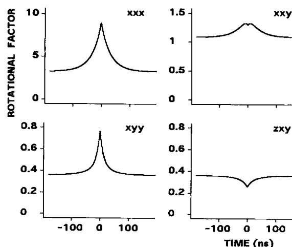
FIGURE 5 The rotational factors of a rigid molecule (theoretical calculations).
